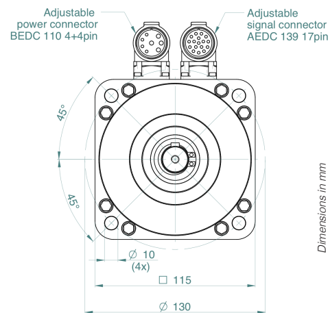
Power connector 4+4 PIN M23 turnable BEDC 110 - Signal connector 17 PIN M23 turnable AEDC 139
