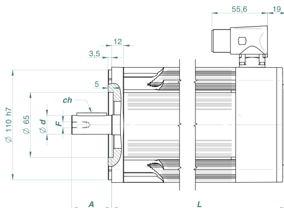
Power connector 4+4 PIN M23 turnable BEDC 110 - Signal connector 17 PIN M23 turnable AEDC 139
